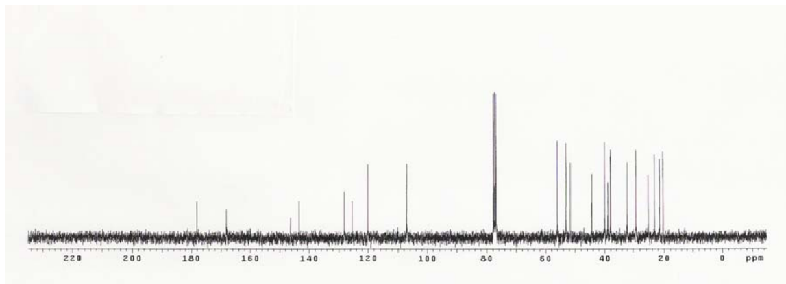
Figure 40: ^{13}\text{C} -NMR Spectrum of Compound 26
