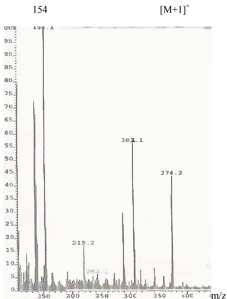
Figure 50: Mass Spectrum of Compound 27
