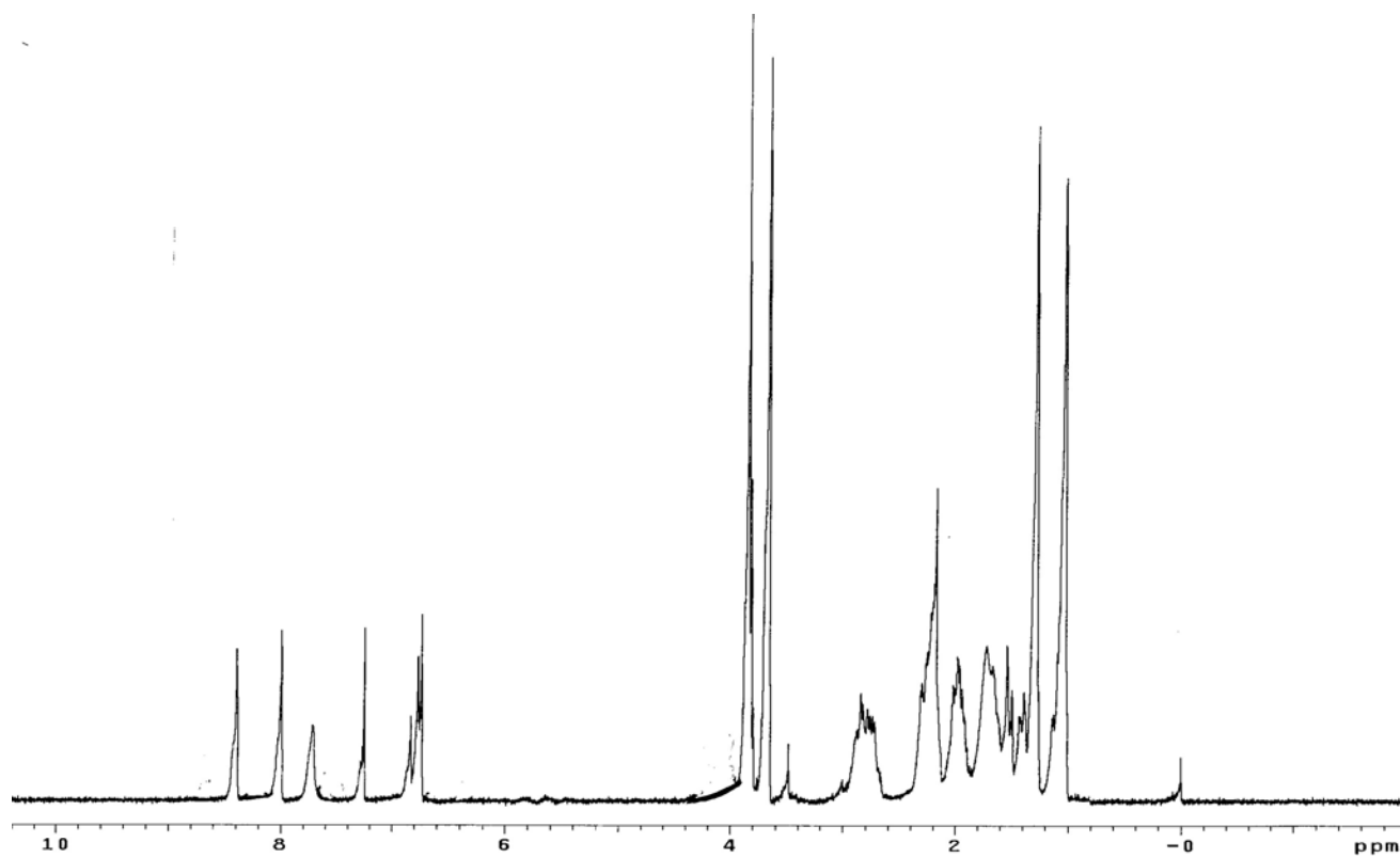
Figure 30: 1 H-NMR Spectrum of Compound 25
