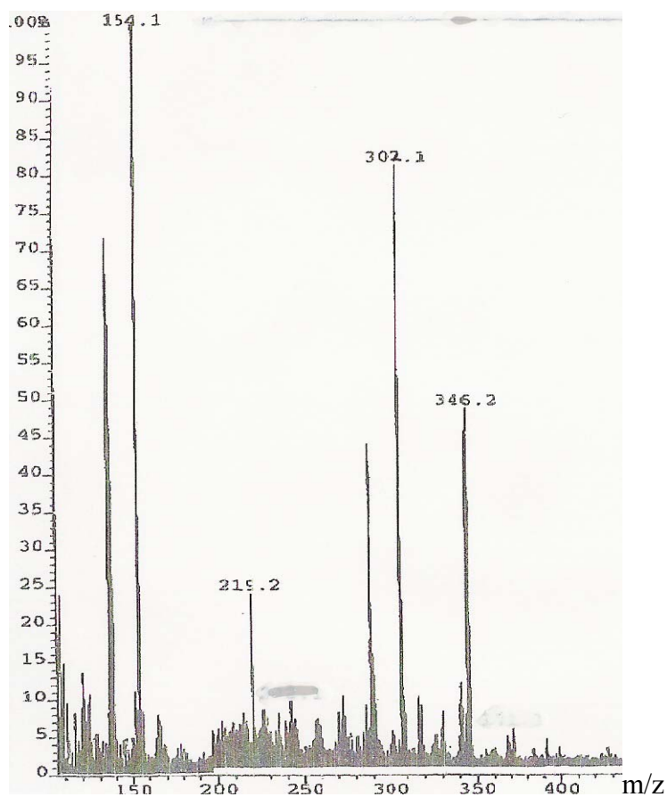
Figure 34: Mass Spectrum of Compound 25
