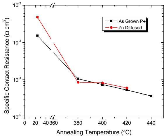
Figure 3.9 Specific contact resistance as a function of processing temperature for p-type contacts.
