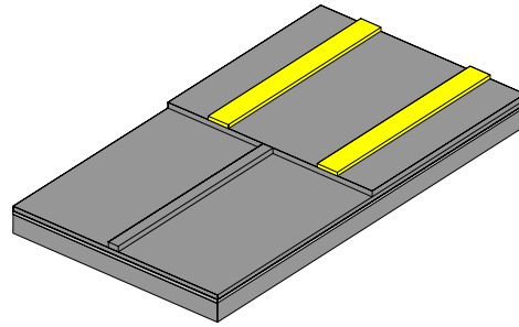
(f) Delineation of input waveguide
