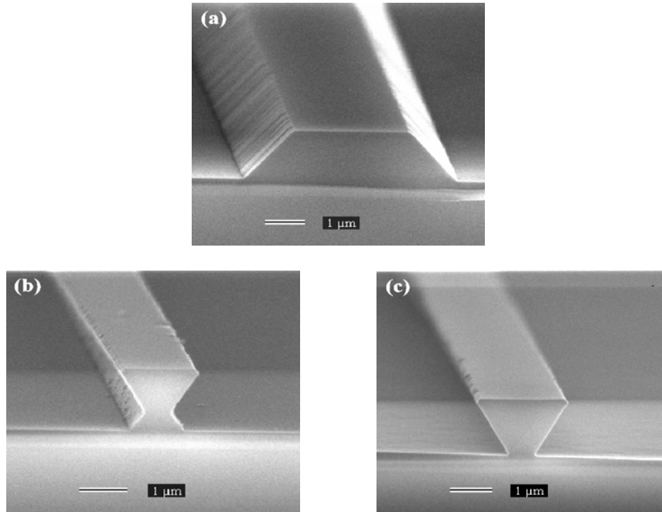
Figure 3.2 HBr based InP wet etching profiles (a) Waveguide along the [1\bar{1}0] direction, (b) Waveguide along the [110] direction, and (c) Over-etched waveguide along [110] direction.
