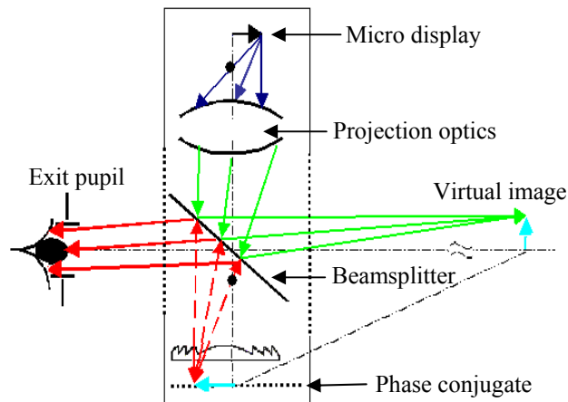
Figure 10: Conceptual design
