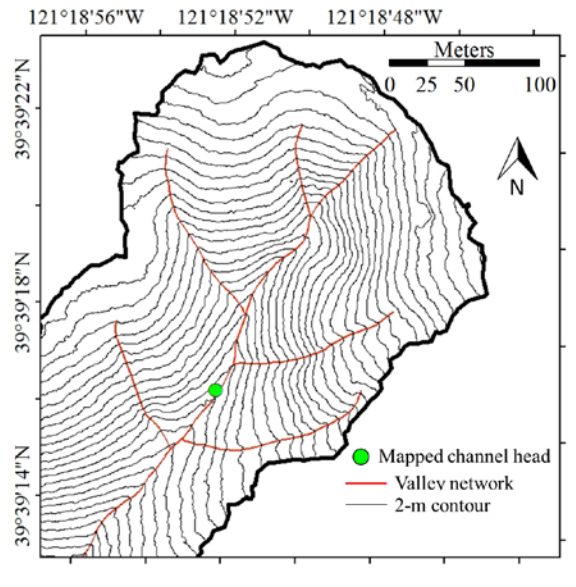
Figure 13. Example of mapped channel heads located in the 2nd-order predicted valley in a subcatchment of Feather River. The presence of contour crenulations suggests the existence of channels upstream of the mapped head.
