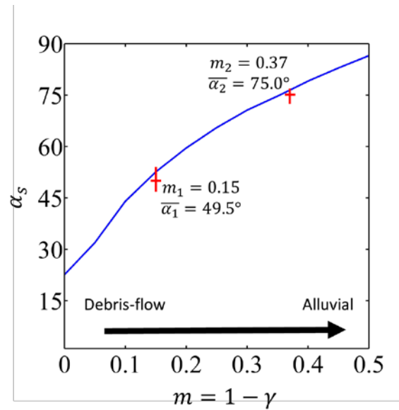
Figure 44. \alpha_s for different values of m = 1 - \gamma , where m is the exponent of slope-area relationship ( S \propto A^{-m} ). The crosses represent the characteristic angles for debris-flow dominated and fluvial regimes based on the observations in the study catchments. The vertical line at each point correspond to the range of the characteristic angles quantified using different approaches (GMM, angle-area curve and slope-area curve; see section 4.1) and reflects the uncertainty.
