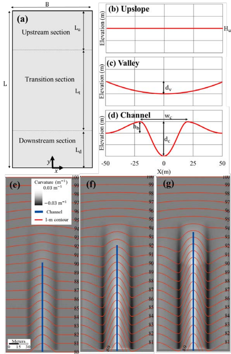
Figure 7. (a) Location of upslope (b), valley (c), and channel (d) cross-sections in the synthetic DEMs. (e), (f), and (g) Curvature and 1-m contours for synthetic DEMs. The numbers are the contour elevations in meters. The imposed channel cross-sections with well-defined banks resulted in sharp signatures in contours as highlighted by the dark background color (negative curvature).
