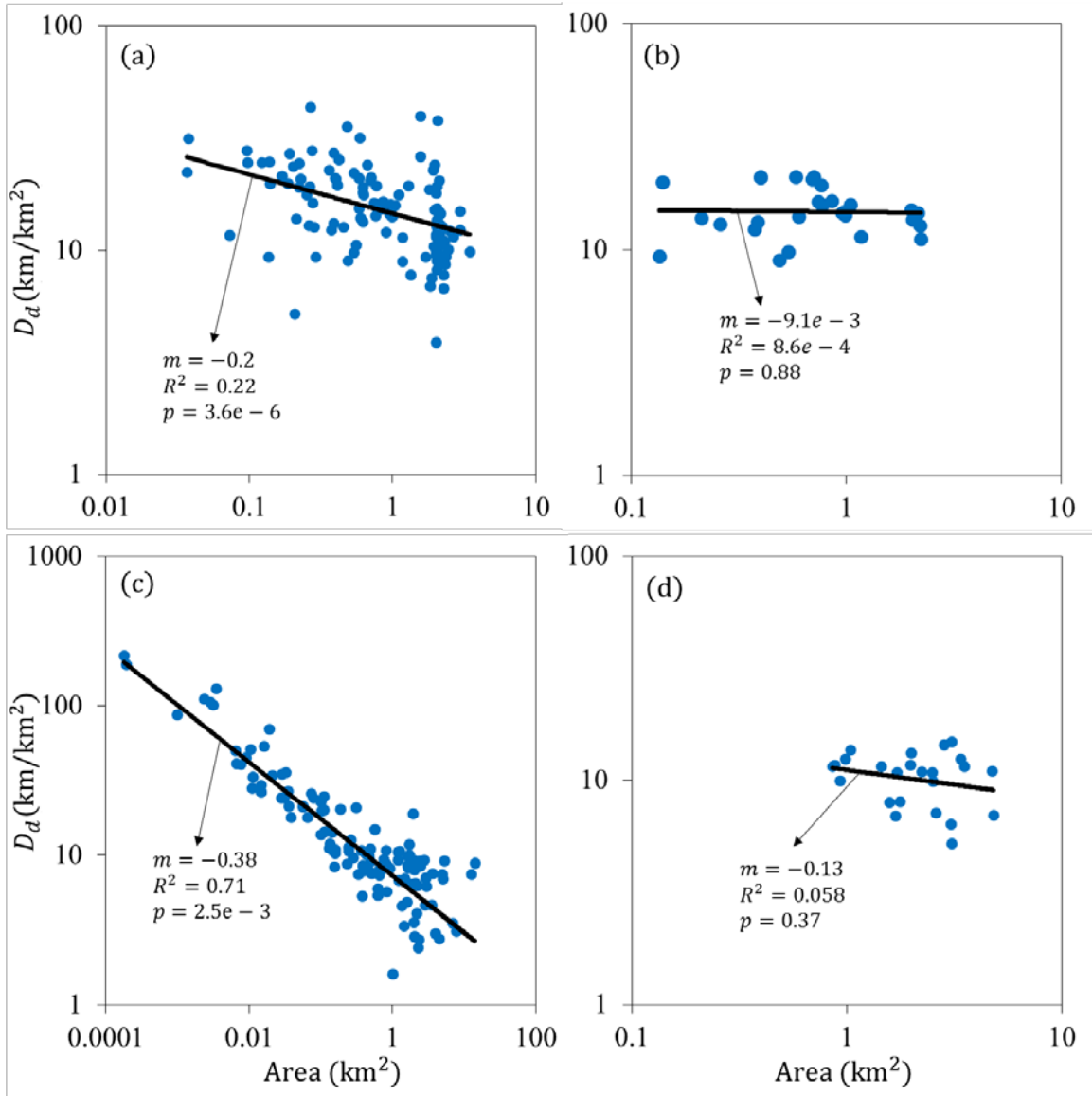
Figure 38. The relationship between drainage density ( D_d ) and drainage area for (a) arid and (b) humid watersheds in this study, (c) watersheds in the arid climate from Melton [1957] , and (c) watersheds in the humid climate from Madduma Bandara [1974]. The least-squares regression line, slope ( m ), R-squared ( R^2 ), and p-value ( p ) are shown.
