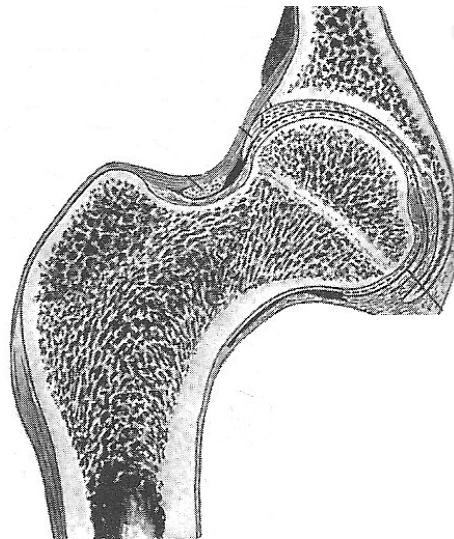
Figure 11. A slice of a human hip joint indicating the varying cortical shell, proximal cancellous bone structure, and medullary cavity
