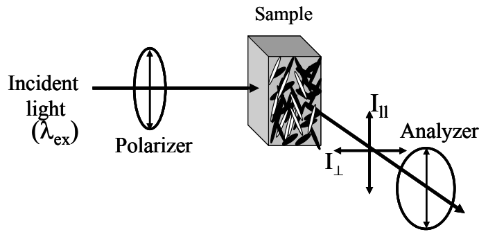
Figure 3.1: Simplified schematic of spectrofluorimeter. As shown polarizer for excitation source and analyzer for emission are in vertical positions ( v ) resulting in the I_{vv}(\lambda) measurement.
