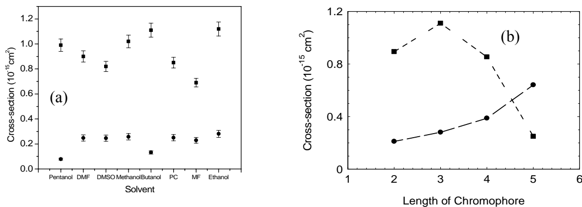
Figure 6.17: Analysis of ground and ESA cross-sections. (a) Ground (squares) and excited-state (circles) cross-section for PD1952 in all host solvents. (b) Peak ground-state cross-section (squares) and excited-state cross-section (circles) as a function of conjugation length (di: DP2350, tri: PD3428, tetra: PD824, penta: PD1659), all dyes in methanol.
