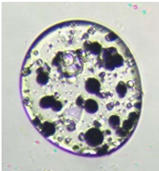
Figure 4 - Micrograph of water-oil-water emulsion droplet containing microscale magnesium particles.
