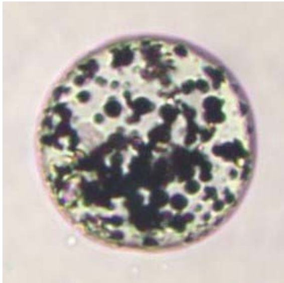
Figure 3 - Micrograph of water-oil-water emulsion droplet containing microscale iron particles.
