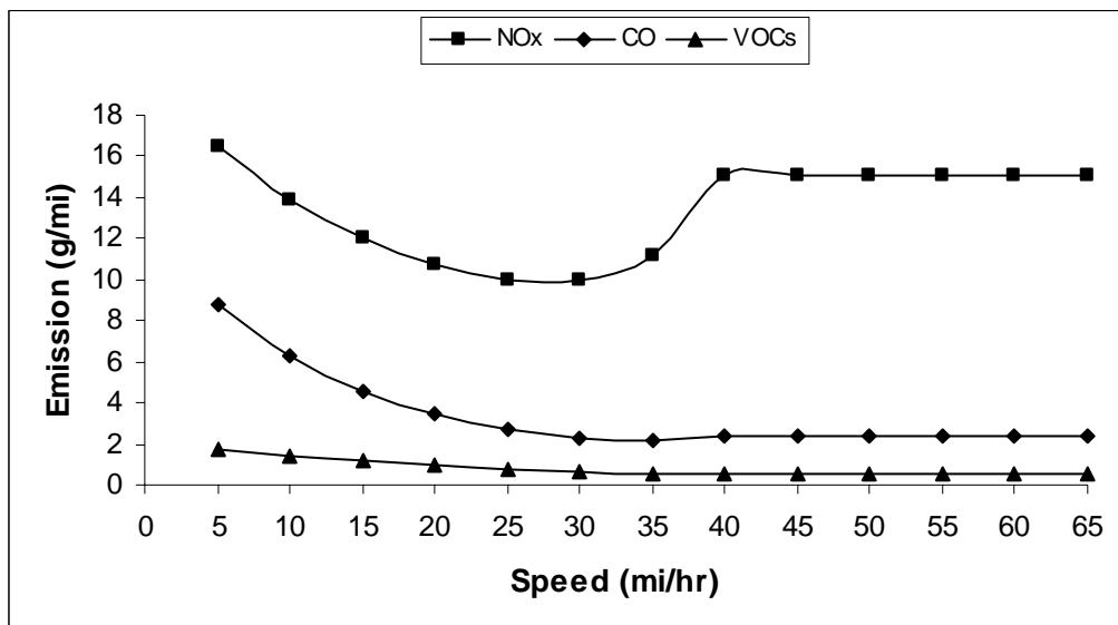
Figure 2-6: Speed sensitivity analysis for school buses, road type arterial
