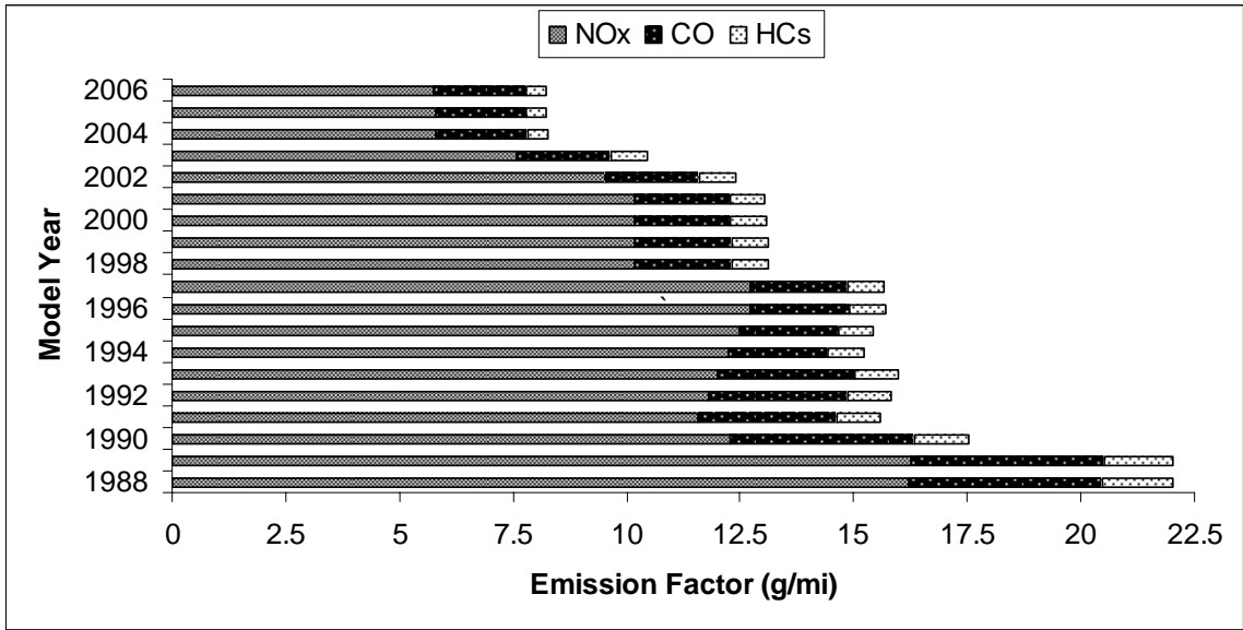
Figure 2-9: The effects of CD and ULSD on NO x , CO, HC s emissions (for both CD and ULSD, model has shown the same result)
