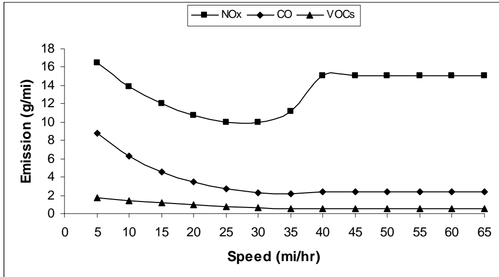
Figure 3-1: Speed sensitivity analysis for school buses, road type arterial
