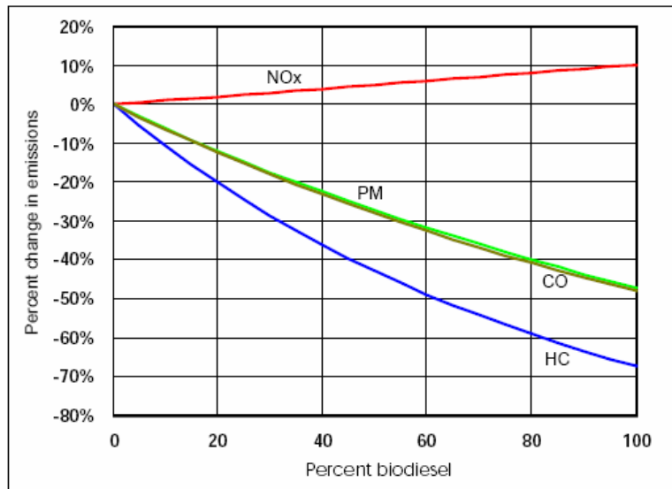
Figure 2-8: EPA reported emissions percentage changes for biodiesel relative to conventional petroleum diesel
