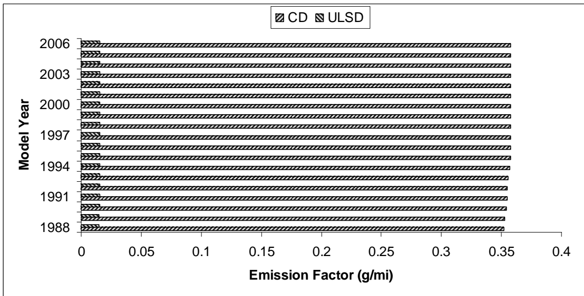
Figure 2-11: The effects of CD and ULSD on SO 2 emissions
