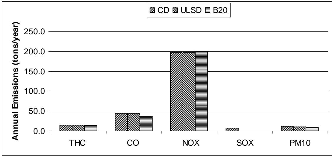
Figure 2-12: The annual emissions from OCPS fleet for different fuels
