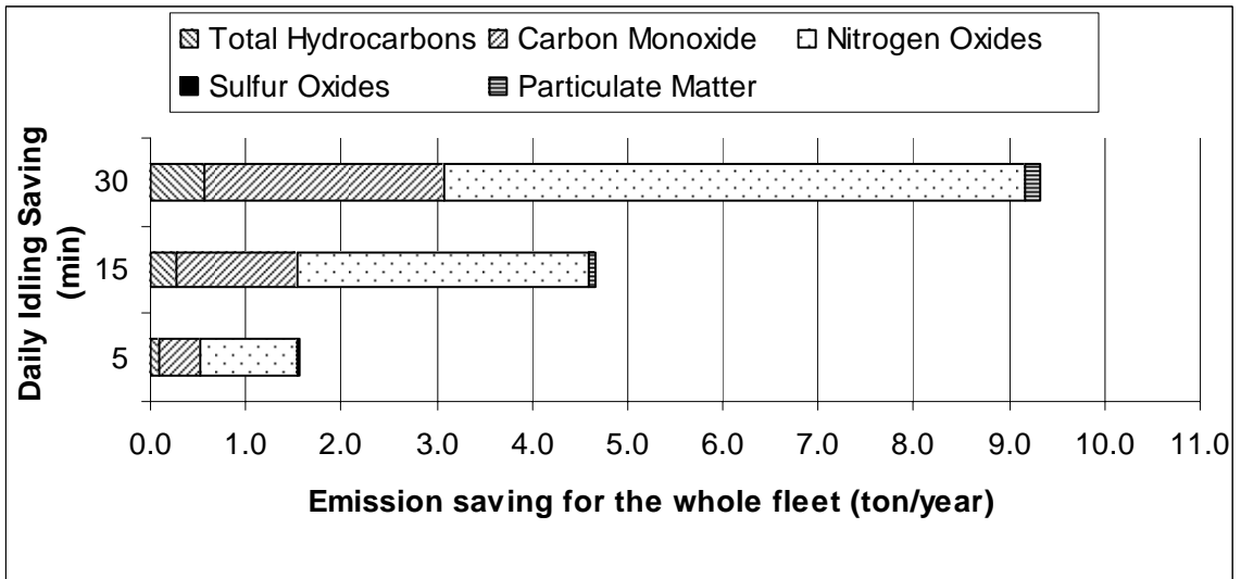
Figure 2-15: The annual emission saving resulted from reduction of school bus fleet idling time for B20
