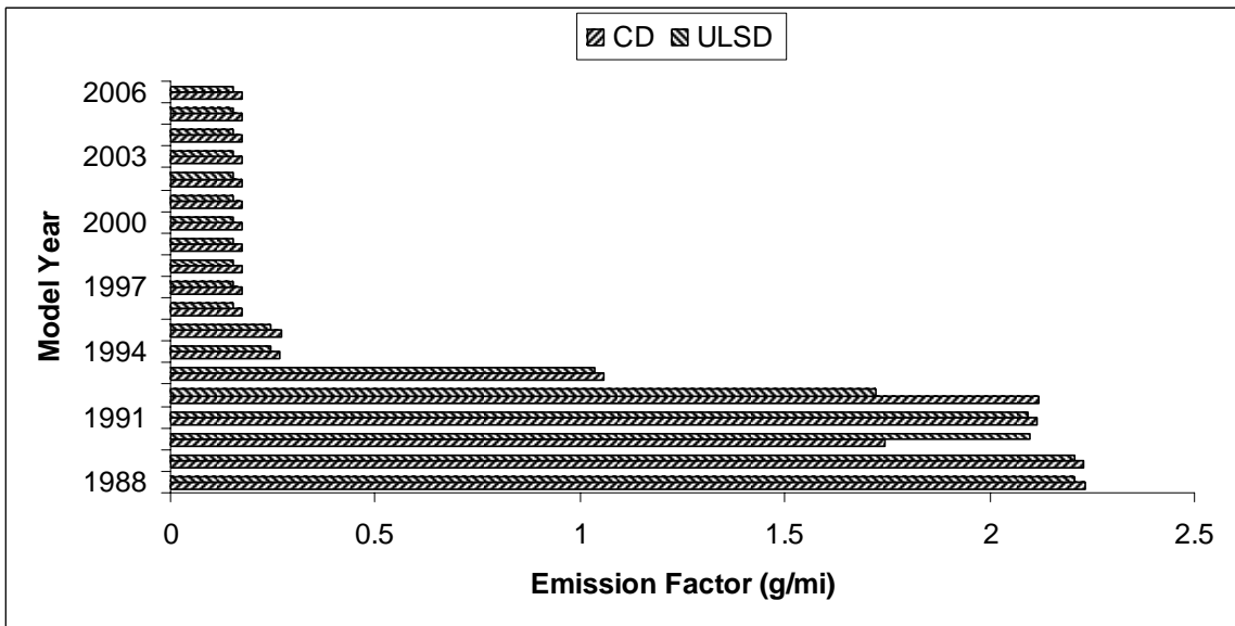
Figure 2-10: The effects of CD and ULSD on PM 10 emissions
