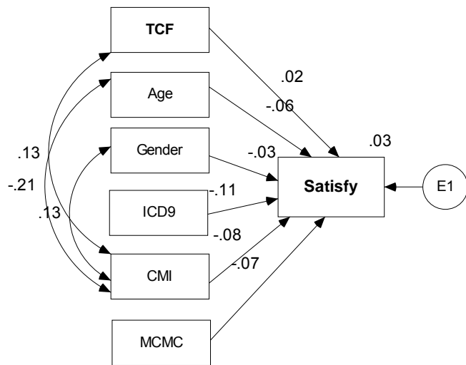
Figure 18: Modified Analytic Path Model for Satisfaction with GOF Measures
