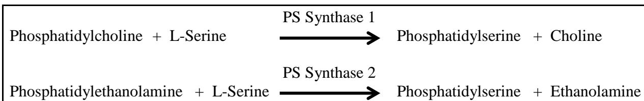
Figure 2: Phosphatidylserine Synthesis
