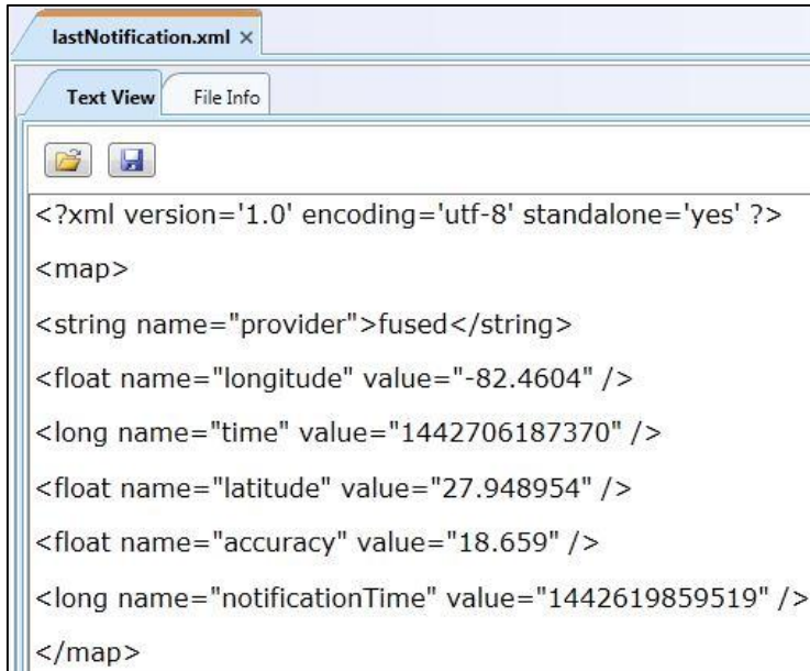
Figure 13 - Content of the Field Trip app's "lastNotification.xml" file
