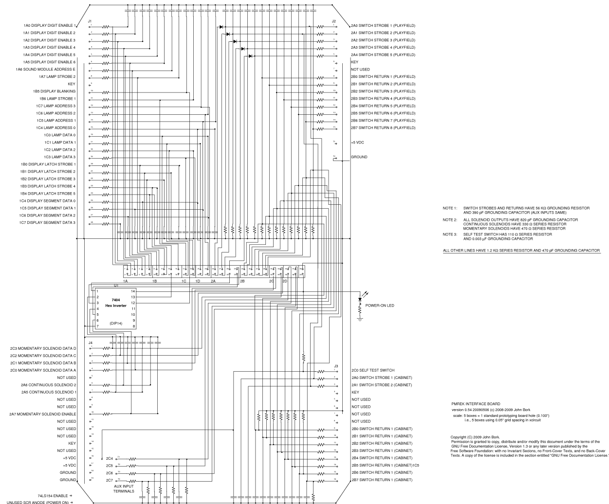
Figure 10: Pmrek Interface Circuit Board to Existing Wiring
