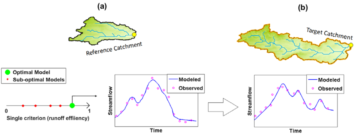
Figure 16. Application of single-objective calibration to runoff efficiency; a) from multiple potential models (red points) the model with greatest NSE is selected as optimal (green point); b) the optimal model selected from the reference catchment is transferred to the target catchment(s) for prediction.
