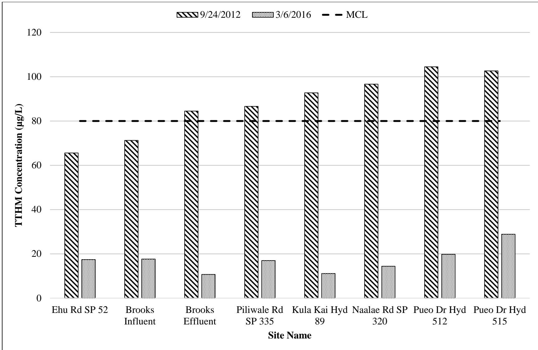
Figure 13: Lower Kula Distribution System TTHM Formation Comparison Analysis
